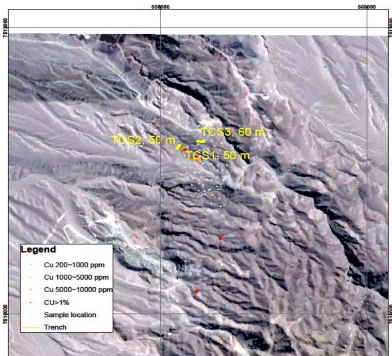
(Figure3) Santa Rosa trench location
